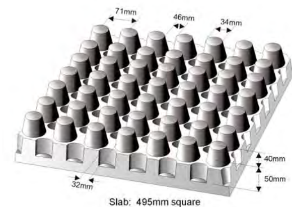
Figure 5.6 “Pelcar” concrete substrate
