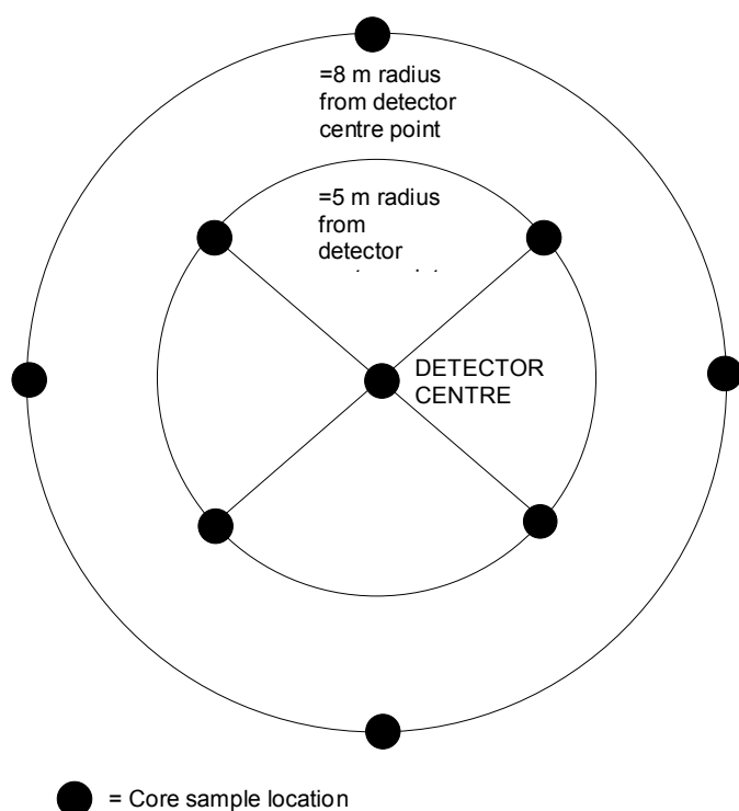
Figure 3.6 – Soil core locations in relation to the detector
