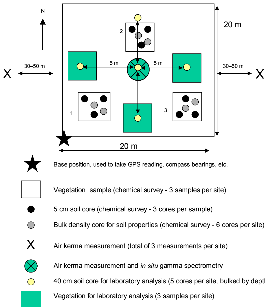
Figure 3.2 – Rural and urban site layout with radiometrics
