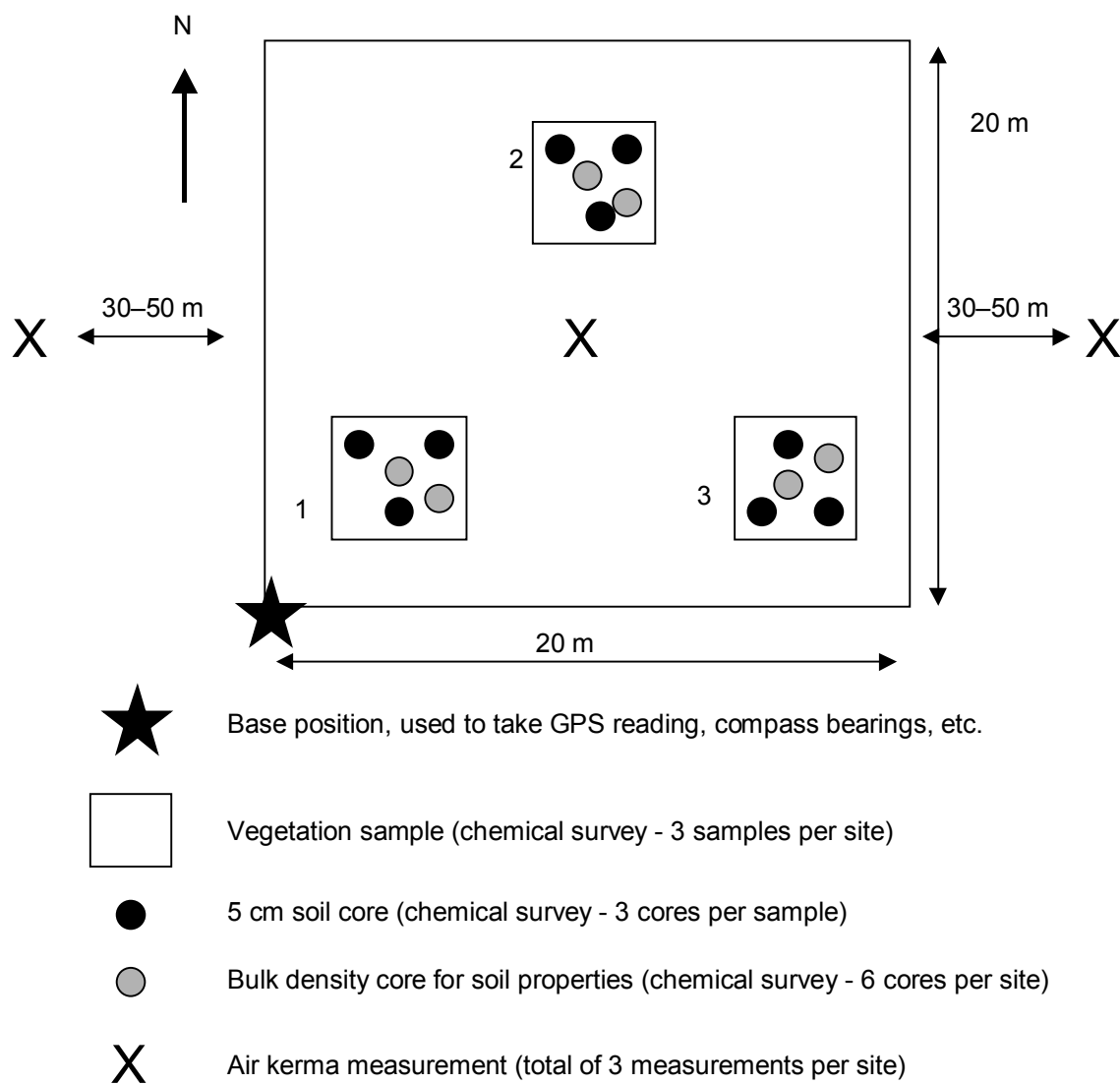
Figure 3.3 – Rural and urban site layout without radiometrics
