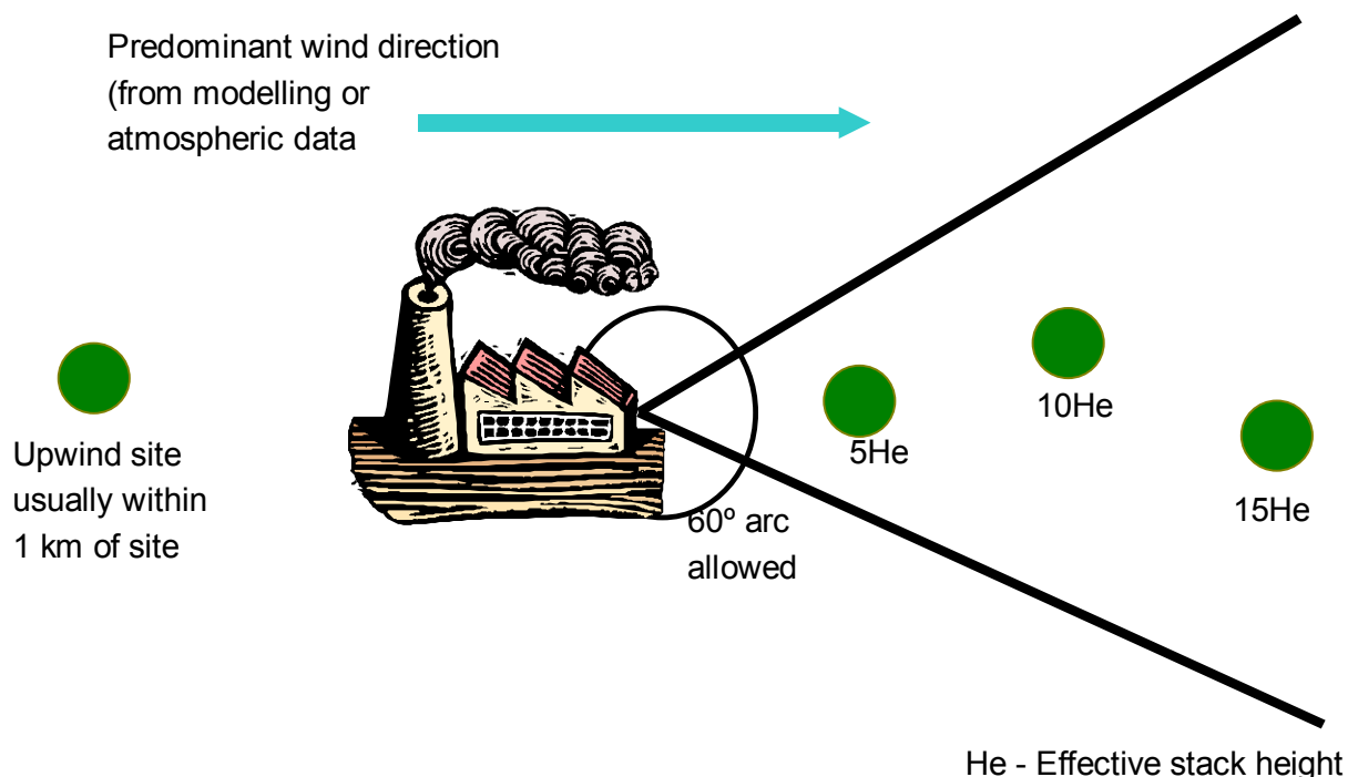
Figure 3.1 – Location of industrial sampling points around industrial site
